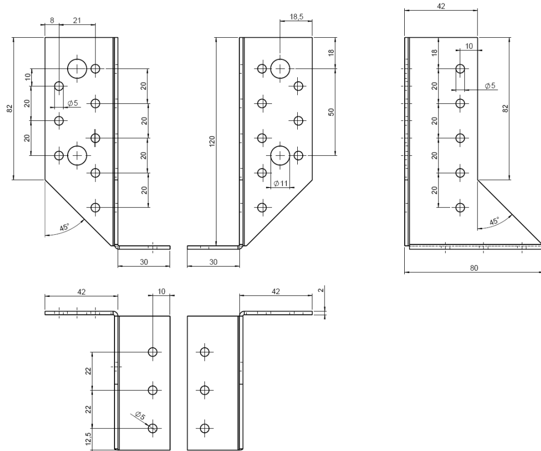
Drawing: Size 30 x 120, 2,0 mm steel
